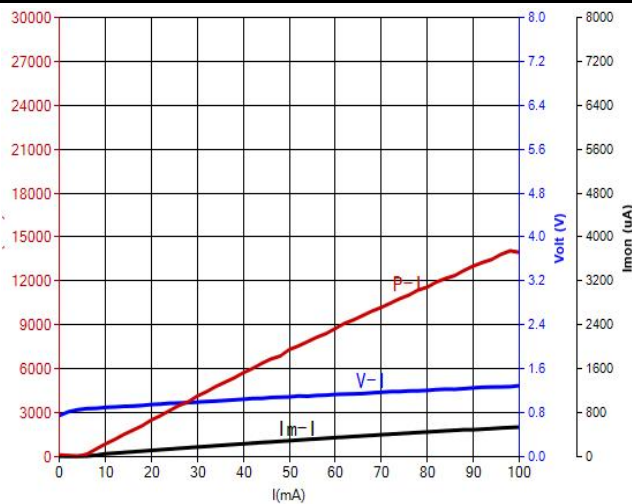
PIV Curve
